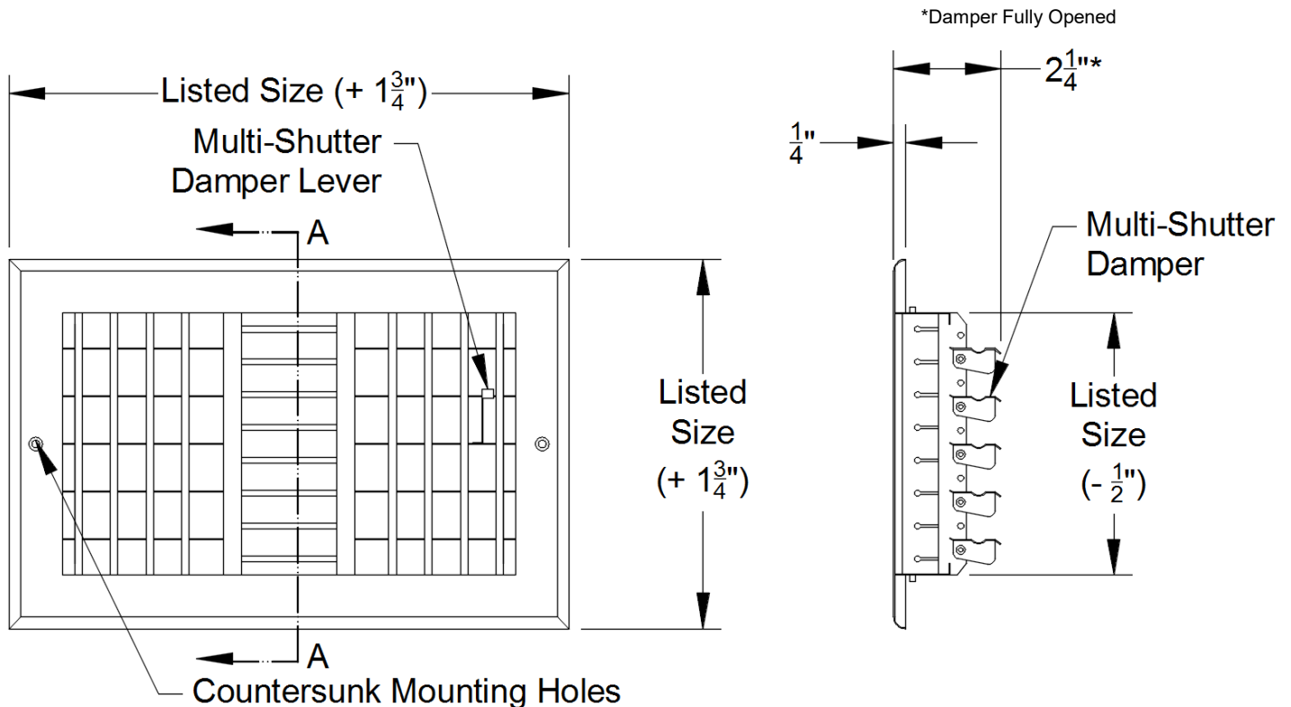
Section AA
