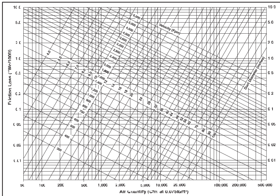
This chart is to be used in place of the standard friction loss chart published in the ASHRAE Handbook of Fundamentals. For conversion of round equivalents to rectangular sizes, use Table 2 "Equivalent Rectangular Duct Dimensions" from the same reference. Test conducted in accordance with TMA AHS-152T.
